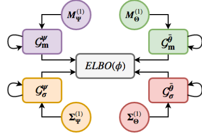
Figure 2: Inference Network Architecture. M_{\mathbf{x}}^{(1)} and \Sigma_{\mathbf{x}}^{(1)} represent the initial learnable embeddings that are used by the respective GRUs \mathcal{G}_m^x and \mathcal{G}_\sigma^x . The output of all GRUs is used to compute ELBO.
