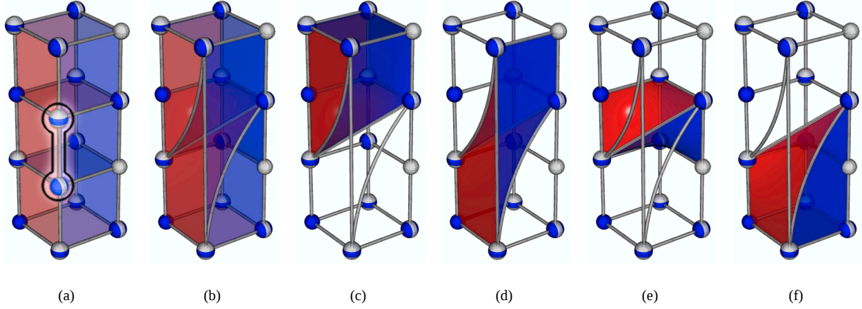
Figure 7: Cells destroyed and created by a saddle-saddle cancellation. The neighborhood of the saddle-saddle pair is divided into four regions of three crystals each and only one region is shown for reasons of clarity. Cells within the other regions are modified in a similar manner. (a) Three crystals before cancellation of the highlighted pair of saddles. (b) Four crystals after cancellation. (c) The top crystal stretches down to the lower 2-saddle. (d) A crystal defined by a new minimum-maximum pair stretches from the lower left to the upper right corner of the region. (e) The middle crystal shrinks after losing the saddle-saddle pair. (f) The bottom crystal stretches up to the 1-saddle on the upper right.
