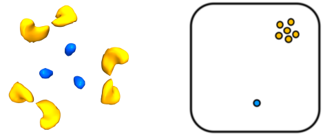
Fig. 3. Mapping contours to points in a descriptor space. Symmetric contours shown in blue are mapped to the same blue point in the descriptor space. Six approximately symmetric contours shown in gold are mapped to six points that lie in close proximity to each other in the descriptor space.
