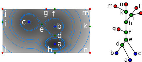
Fig. 2. The contour tree captures changes in the topology of the level sets of a scalar field. (left) A scalar field and its level sets. (right) The corresponding contour tree. The red nodes are local maxima, the blue nodes are local minima, and the green nodes are saddles.
