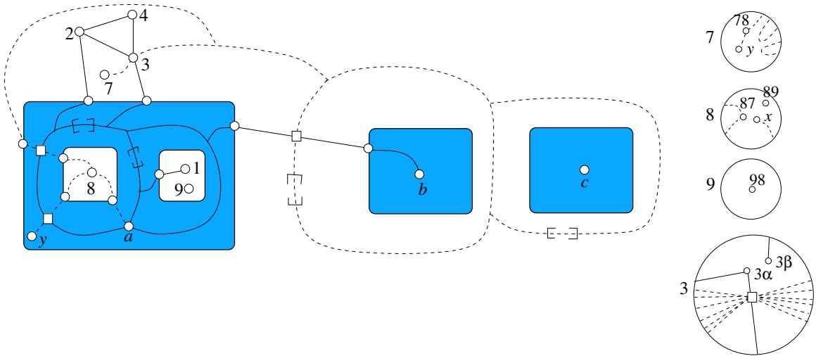
Figure 3.26: Extending ascending disks: The three A-paths are extended towards the highest vertices in the appropriate continents using the path to the root in the shortest path tree. This introduces new paths in the normal disks of 7, 8, and 3. A spike is introduced to prevent an illegal intersection between one of the descending disks starting at p and the ascending disk represented by the A-path between y and 8. This spike is represented within the normal disk of 7 by the path between base points 78 and y .
