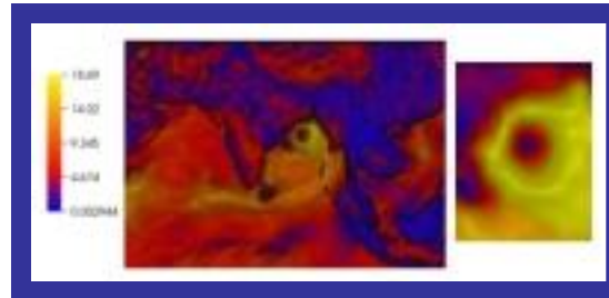
Fig: Windspeed visualization
