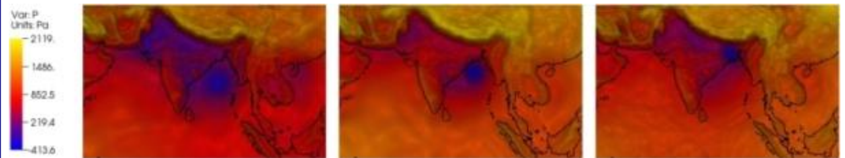
Fig: Volume Rendering (using VisIt ) of Perturbation Pressure output from WRF at 18:00 hours on 23 rd , 24 th and 25 th May 2009
