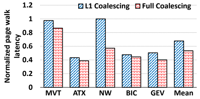
Fig. 11: Normalized average page walk latency with coalescing.
