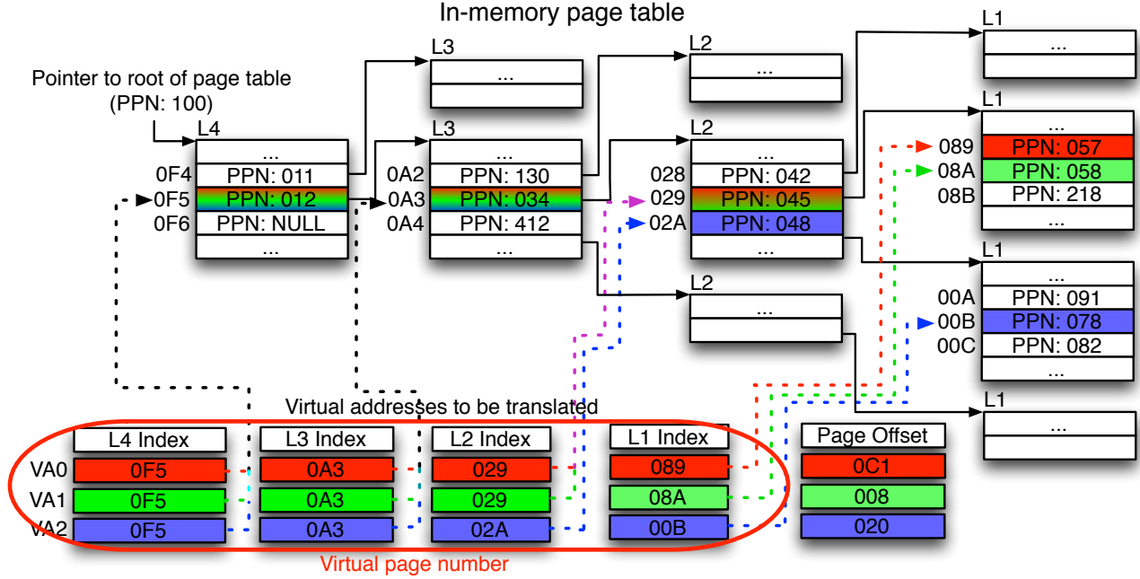
Fig. 2: Example page walks of three different virtual page addresses (colored red, green and blue).
