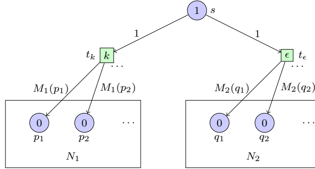
Fig. 8. Constructed Petri net N
