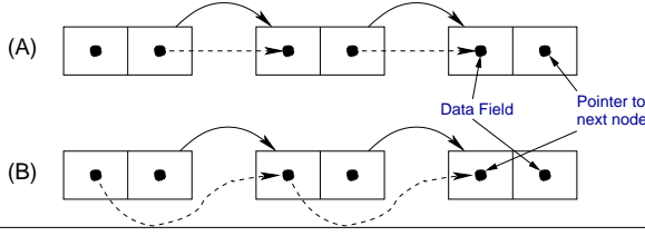
Figure 3. An example showing the different levels of granularity at which the heap-graph can be constructed. Dotted lines show the heap-graph constructed at field-granularity, while bold lines show the heap-graph constructed at object-granularity.
