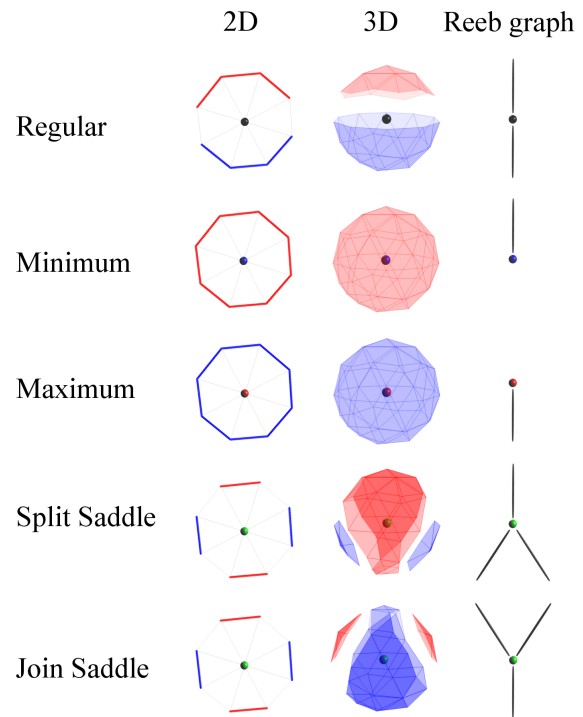
Fig. 2. Classifying a vertex as regular, minimum, maximum or saddle using the topology of its local neighborhood. The lower link of a vertex is colored blue; its upper link is colored red. The structure of the Reeb graph is shown in the right column. The connectivity of the level sets further classifies the saddle as a split or join saddle.
