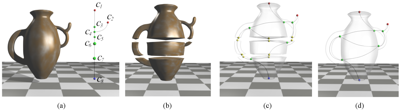
Fig. 5. The Reeb graph computation algorithm. (a) The join tree for the input is computed and the loop saddles are identified. Here, c_6 and c_7 are identified as loop saddles. (b) The input is split at a function value infinitesimally above that of the loop saddles to obtain a set of interval volumes. (c) The contour tree for each interval volume is computed. (d) The contour trees are merged to obtain the Reeb graph of the input.
