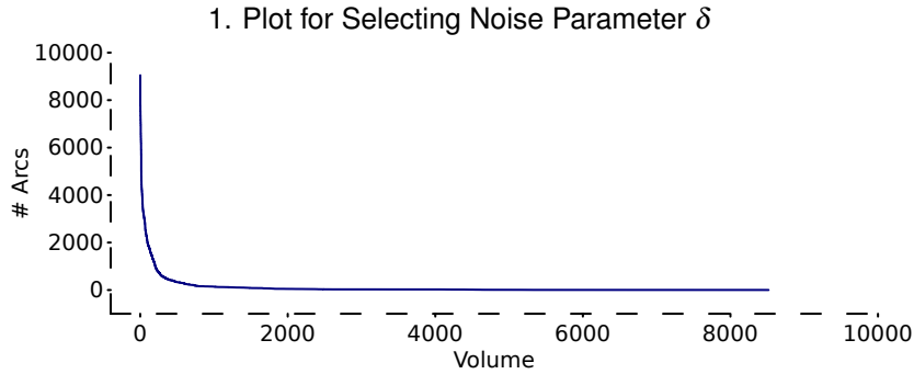
Fig. 1. The plot of the number of arcs in the contour tree with a specific value of volume as the value of the volume increases. The curve shows a significant drop initially due to the arcs corresponding to noise. A value immediately after this drop is chosen as the value of \delta . The above plot corresponds to the Fuel dataset. Plots corresponding to the other datasets behave similarly.
