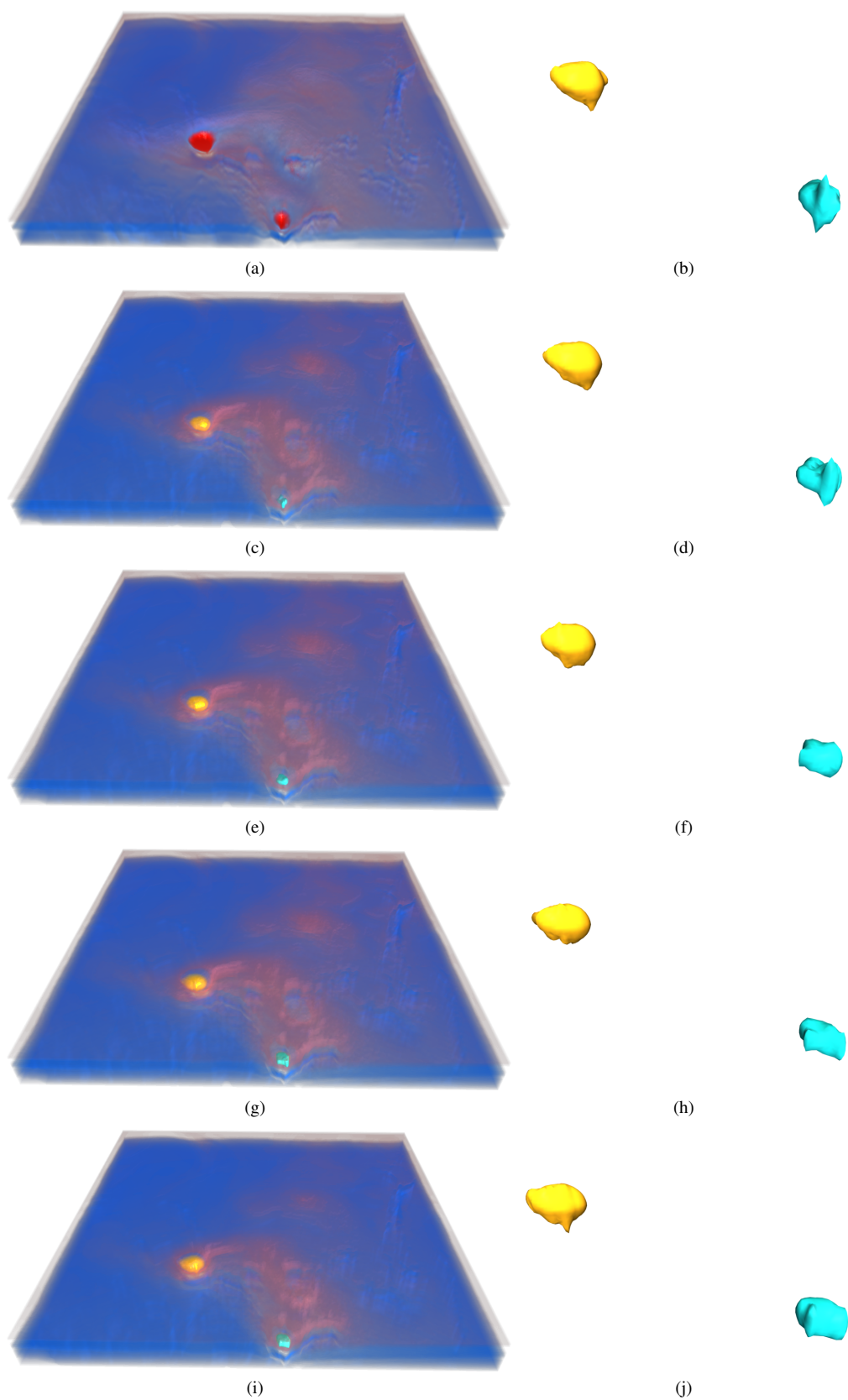
Fig. 4. Query contour driven exploration using multiple contours on a weather simulation dataset of size 306 \times 285 \times 27 . (a) Volume rendering of the pressure field from the first time step of the simulation shows two depressions in the Pacific ocean in red. (b) Two query contours selected from the low pressure region of the first time step shown in gold and cyan. (c)-(j) The result of the query on four subsequent time steps that are one hour apart shows the two low pressure regions detected in gold and cyan. The left and the right columns show the volumetric region extracted and the contour located, respectively.
