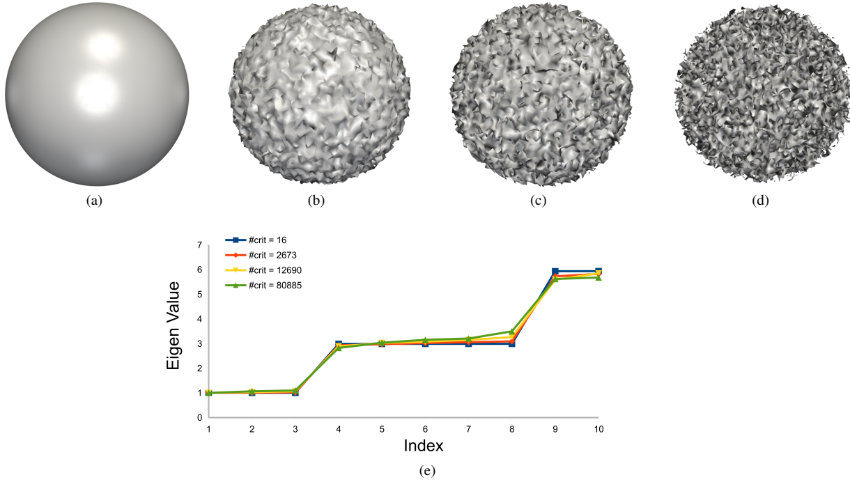
Fig. 6. Robustness to noise. (a) An isosurface of a synthetic dataset which has the shape of a sphere. The number of critical points for this dataset is 16. (b)-(d) Adding increasing levels of noise to the dataset deforms the isosurface. The number of critical points increase to 2673, 12690, and 80885. (e) For each datasets, the first ten non-zero eigen values of the Laplace-Beltrami spectra are normalized by dividing with the first non-zero eigen value and plotted as a 1D curve. The similarity of the curves shows that the similarity of the contours can be identified easily even in the presence of noise.
