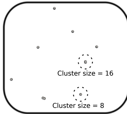
Fig. 2. Projection of 93 points in the descriptor space to 2D using multidimensional scaling for the dataset EMD-1654. Observe that the clusters are well separated. For the two clusters within the dotted circles, their sizes are annotated below the cluster.
