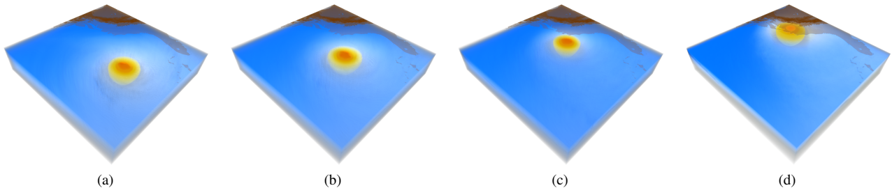
Fig. 3. Low pressure regions extracted through query contour driven exploration of the hurricane Isabel dataset. The yellow regions highlight the volumetric regions identified from the time steps, 12, 24, 36, and 48, using the query contour from the first time step shown in Figure 7(c). The extracted regions are displayed in the context of the rest of the volume.
