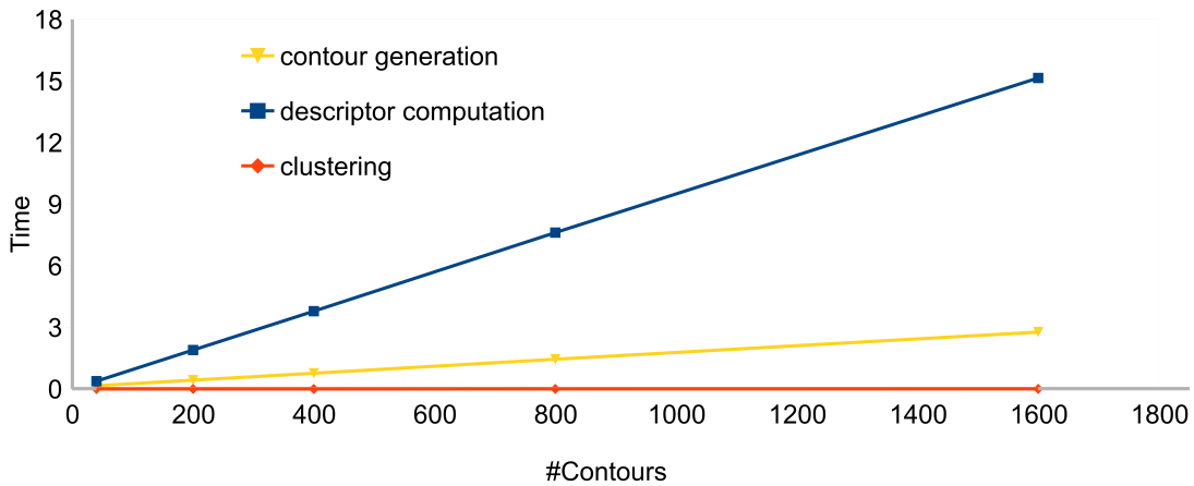
Fig. 7. Computational performance scales linearly with respect to the number of contours. The time taken, in seconds, for contour generation, descriptor computation, and clustering are plotted when the number of contours processed are 40, 200, 400, 800, and 1600. The plot shows linear scale up in the computation time for contour generation and descriptor computation. The nearest neighbour search takes only a fraction of a second. The contours are generated from the dataset EMDB-1654. To limit the variation in performance due to differences in the size of the contours, this experiment was performed with contours belonging to a single scale.
